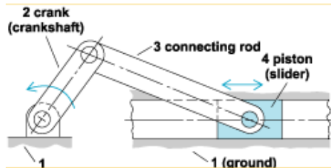
Typical Slider-Crank
