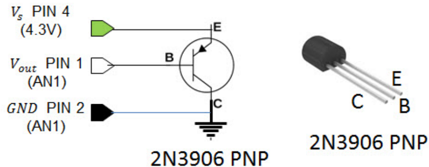
Fig.5-3: The 2N3906 transistor is also a TO-92 package. This particular version (Radio Shack 276-1604) has the 3-pins labeled as shown (right).
